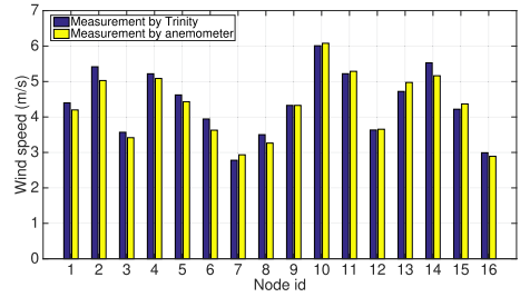
Fig. 21. Average airflow speeds.
