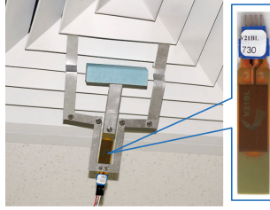
Fig. 3. Energy harvester and its key component bimorph.
