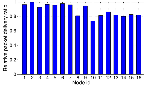
Fig. 19. Relative PDRs between Trinity and CTP.
