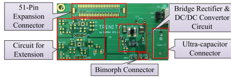
Fig. 4. Power management module.
