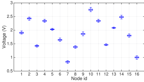
Fig. 20. Voltage readings.
