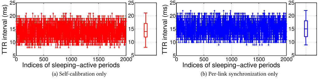
Fig. 17. Performance of Trinity synchronization.
