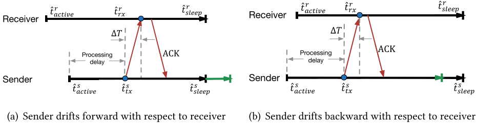
Fig. 10. Per-link synchronization between two nodes. The green arrows denote the original dormant times for the sender before synchronizing with the receiver.
