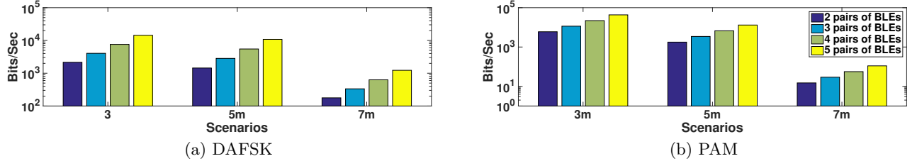
Figure 24: Throughput of up to five pairs of BLE device in nLoS scenario.
