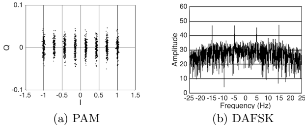
Figure 26: Two modulations produced by BLE and sensed by WiFi using CSI values. By varying the transmission power levels of BLE packets, BLE packets can carry information that can be sensed by WiFi.
