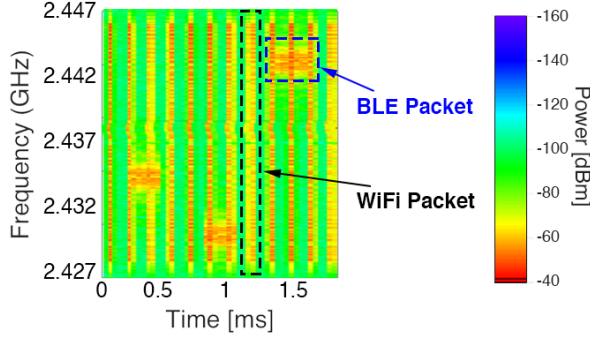
Figure 3: Power Spectral Density of WiFi and BLE
