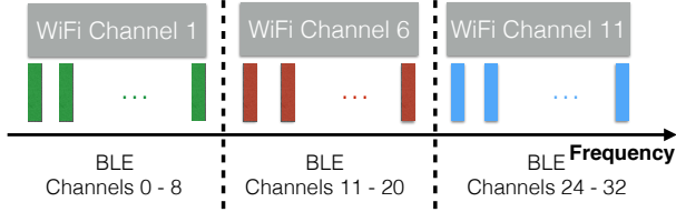
Figure 14: Overlaps of BLE channels with WiFi channels
