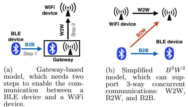
Figure 1: Gateway-based model vs. B^2W^2 model
