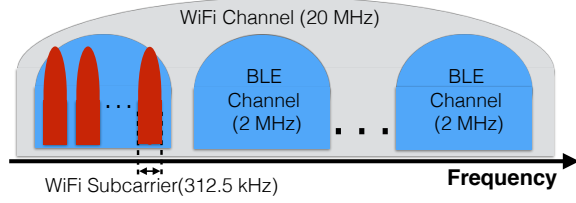
Figure 8: The relationship between a WiFi channel and BLE channels
