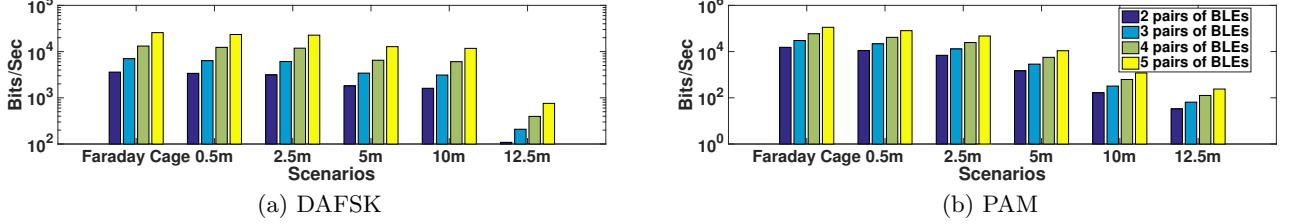
Figure 22: Throughput of up to five pairs of BLE device in LoS scenario.
