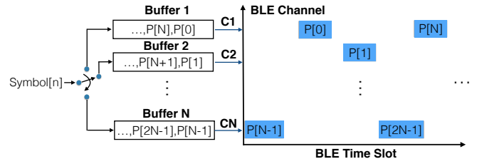
Figure 7: A General Architecture of Symbol Mapper
