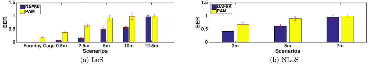
Figure 19: The BER of BLE to WiFi devices communications shows that DAFSK resulted in fewer errors than PAM in both LoS and NLoS scenarios. While PAM has higher throughput, it is more prone to errors in noisy environments.
