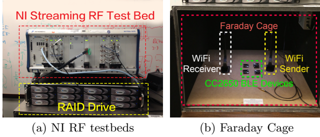
Figure 17: The experiment setup: NI testbeds has the ability to regenerate and process sensed signals to produce CSI. TI CC2650 BLE device varied the BLE power levels to carry information.
