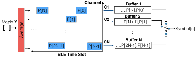
Figure 12: Architecture of symbol reconstructor
