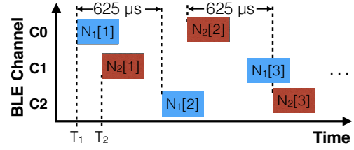
Figure 15: Two BLE networks Tx. to a WiFi receiver
