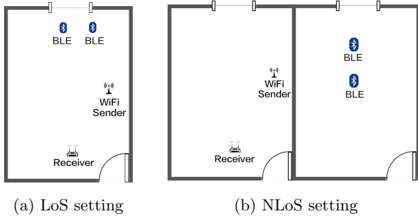
Figure 16: Experiment settings of two scenarios: Direct Line-of-Sight and none Line-of-Sight. We change the distance between the WiFi Sender and BLE devices.
