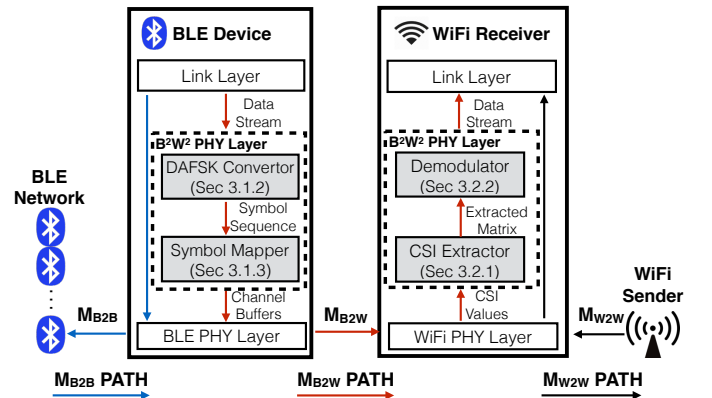
Figure 2: Overview of 3-way concurrent communication
