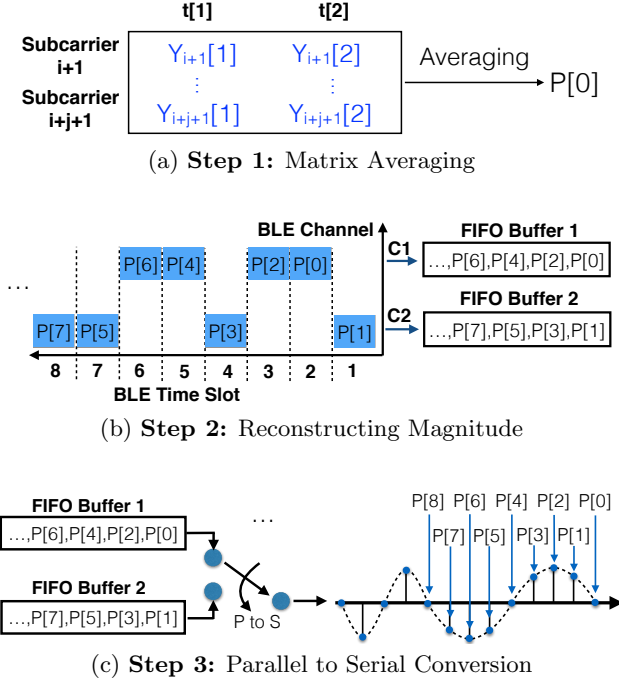
Figure 11: Example of symbol reconstructing with 2 BLE Channels
