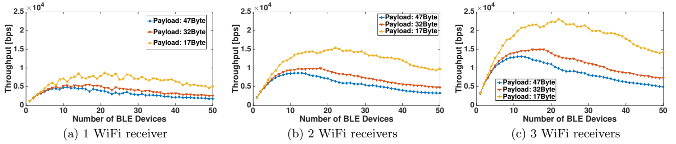
Figure 27: The throughput with different number of BLE senders and WiFi receivers
