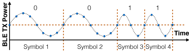
Figure 5: An example of converting "0011" from M_{B2W} message into symbols using the DAFSK converter. Each blue dot represents a BLE transmission power level to be tuned on an outgoing BLE packet.
