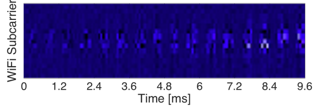
Figure 4: Recovered power level information based on the CSI value changes on the WiFi receiver side. The higher the color, the higher the received BLE signal's power at the WiFi receiver.
