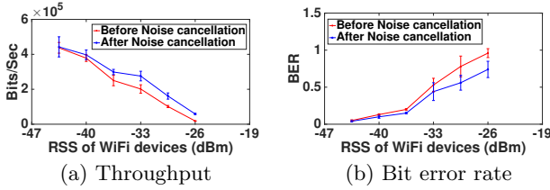
Figure 23: The throughput and BER of BLE to BLE communication show that we are able to cancel out the known WiFi beacons by using a inverted WiFi beacon phase.
