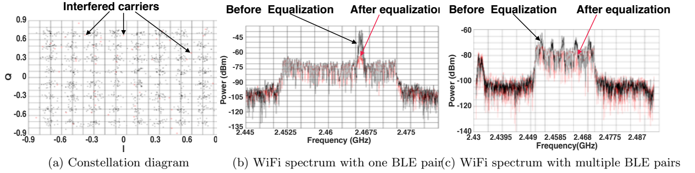
Figure 25: These diagrams show the ability to sense interfered carriers and how the equalization scheme works. The red points in the constellation diagram are interfered carriers. The red colored spectrum demonstrate the effectiveness of the equalization and noise cancelling scheme while the black colored spectrum is the interfered spectrum.
