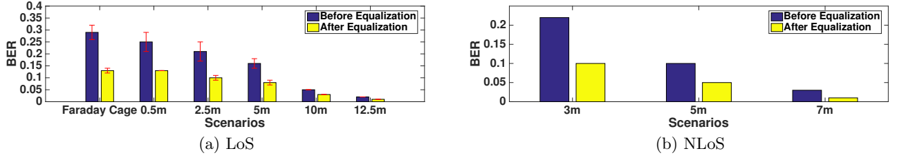
Figure 21: The BER of WiFi to WiFi communications with Bluetooth interference show that the shorter the distance between WiFi and BLE, the higher the BER. We demonstrate by our equalization and BLE cancellation scheme decreases BER by 50% in both LoS and NLoS scenarios.
