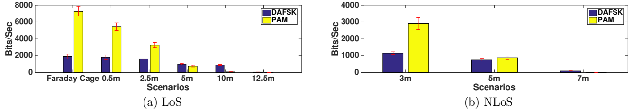
Figure 18: The throughput of BLE to WiFi devices communications in both LoS and NLoS scenarios shows that at close ranges, PAM performance is better than DAFSK. DAFSK maintains throughput better at longer distances.
