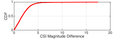
Figure 10: Empirical results to demonstrate the stability of CSI values in frequency domain: between two neighboring subcarriers in frequency domain, 80% of CSI magnitudes have the difference less than 3.
