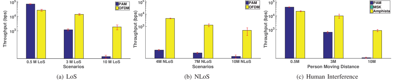
Fig. 13: Z2W Throughput
