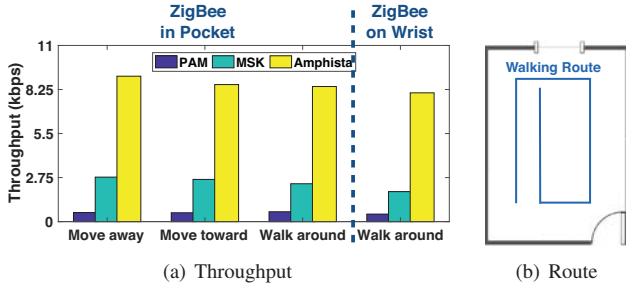
Fig. 14: The performance of ZigBee to WiFi communication in four different mobile scenarios. The throughput error ranged about 15-20% which means our modulation schemes remain robust and against fading caused by human movement.
