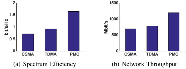
Fig. 24: Spectrum efficiency and network throughput. The spectrum utilization of PMC is 2.3 and 1.8 times higher than CSMA and TDMA approaches, respectively.
