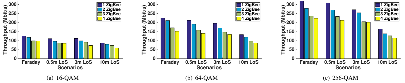
Fig. 19: In LoS scenario, conventional WiFi receiver's throughput in a 40 MHz WiFi channel with different modulation schemes (16-QAM, 64-QAM, and 256-QAM) slightly decrease over distance. When conducting parallel transmission to 1, 2, 3, and 4 ZigBee receivers, conventional WiFi receiver's highest throughput are 319.76 Mbit/s, 278.51 Mbit/s, 235.88 Mbit/s and 223.77 Mbit/s, respectively.
