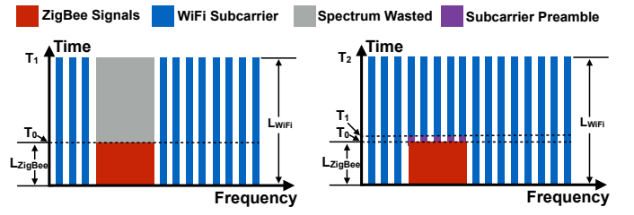
(a) Spectrum wasted issue
