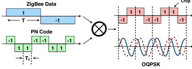
Fig. 6: Example of DSSS process
