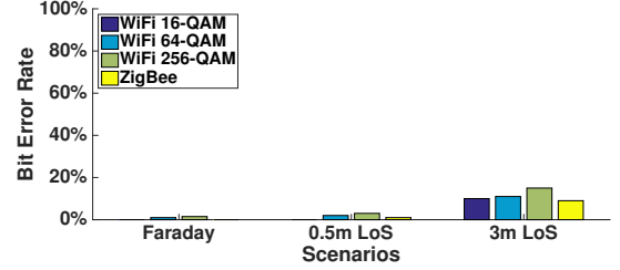
Fig. 23: BER at conventional WiFi and ZigBee receivers.
