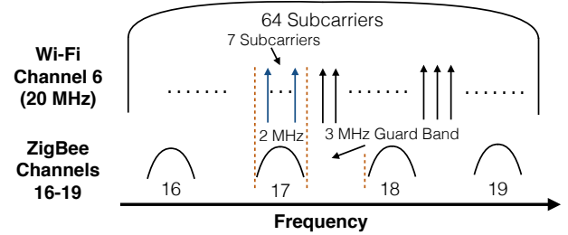
Fig. 2: Overlapped channels of ZigBee and WiFi
